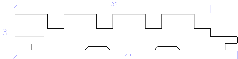
Profile B4
