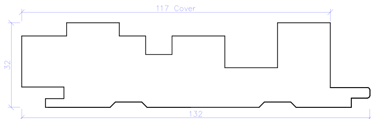
Profile C3
